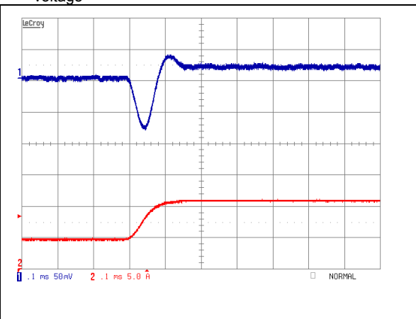
iEA48025A015V-000 Typical transient response. Output voltage response to load step from 50% to 75% of full load with output current slew rate of 0.1A/ \mu S.
